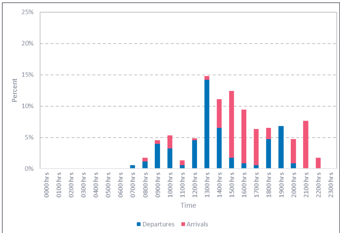
Figure 8: F-35A aircraft distribution of movements per hour: 2023 to 2024, RAAF Base Darwin
