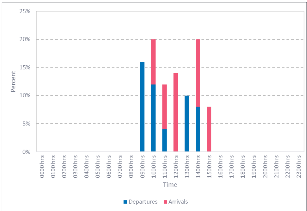
Figure 20: F-35A aircraft operation times: RAAF Base Pearce
