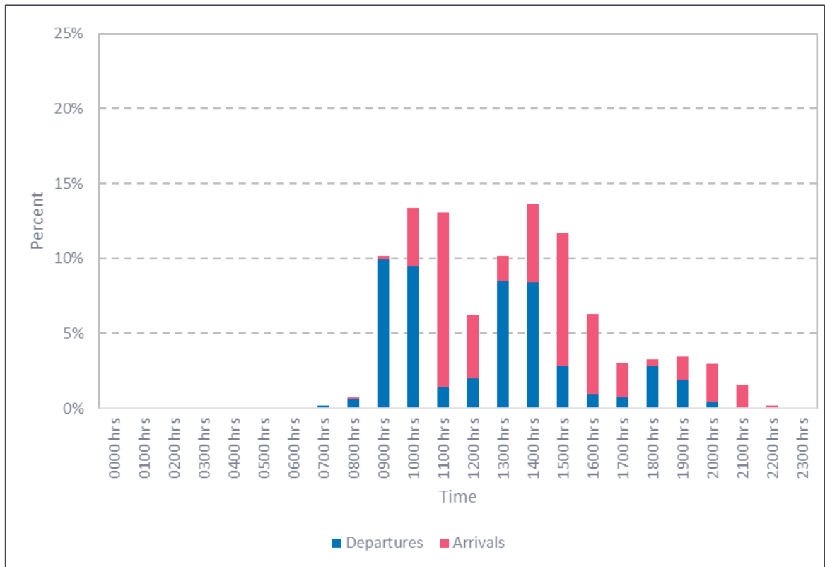
Figure 6: F-35A aircraft distribution of movements per hour: 2023 to 2024, RAAF Base Tindal
