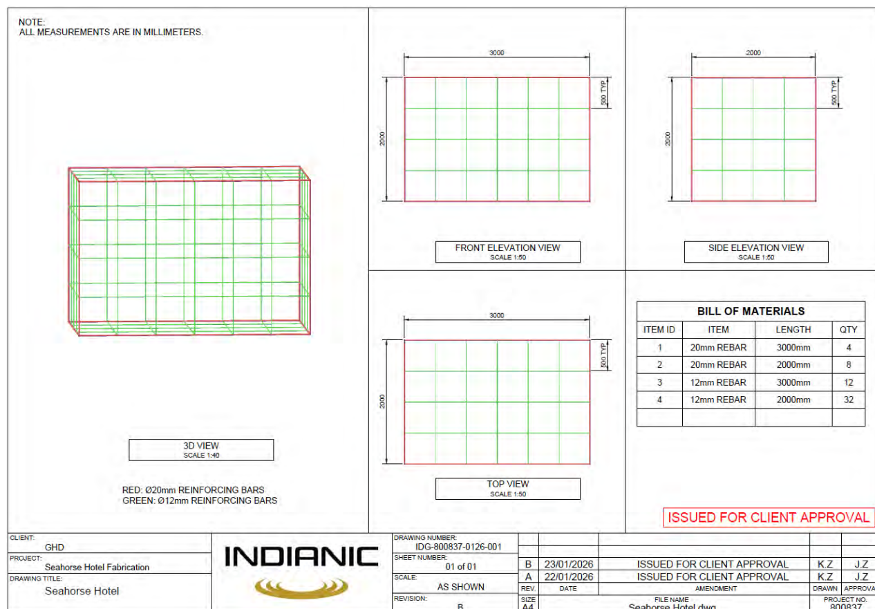
Figure 2-3 Proposed artificial habitat structure
