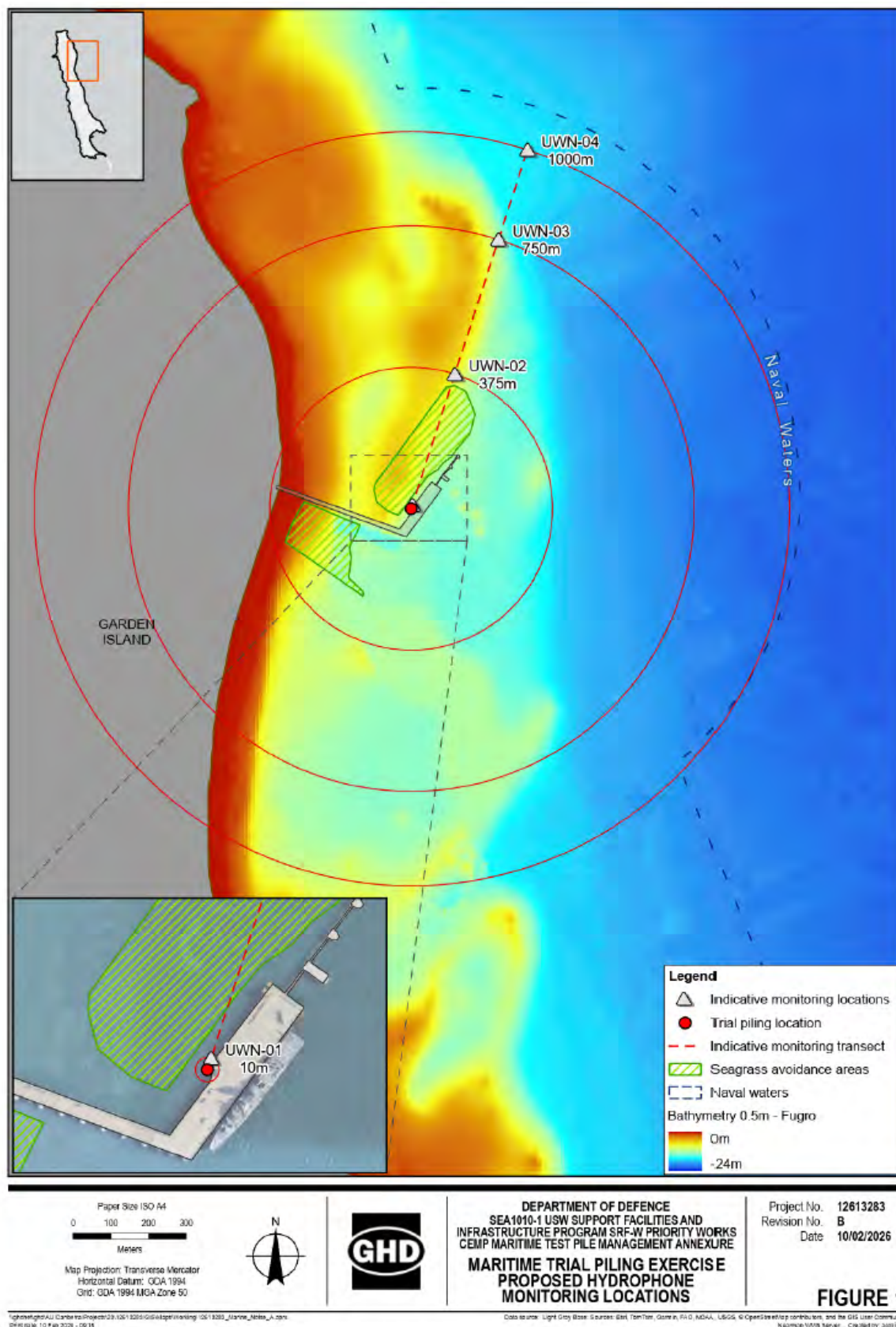
Figure 1 Proposed hydrophone monitoring locations
