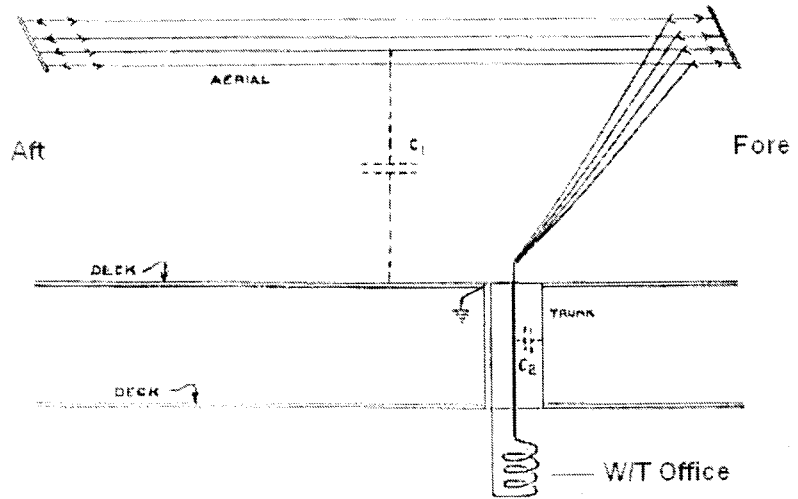
The Inverted L aerial system found on naval ships upto the 1950's.
