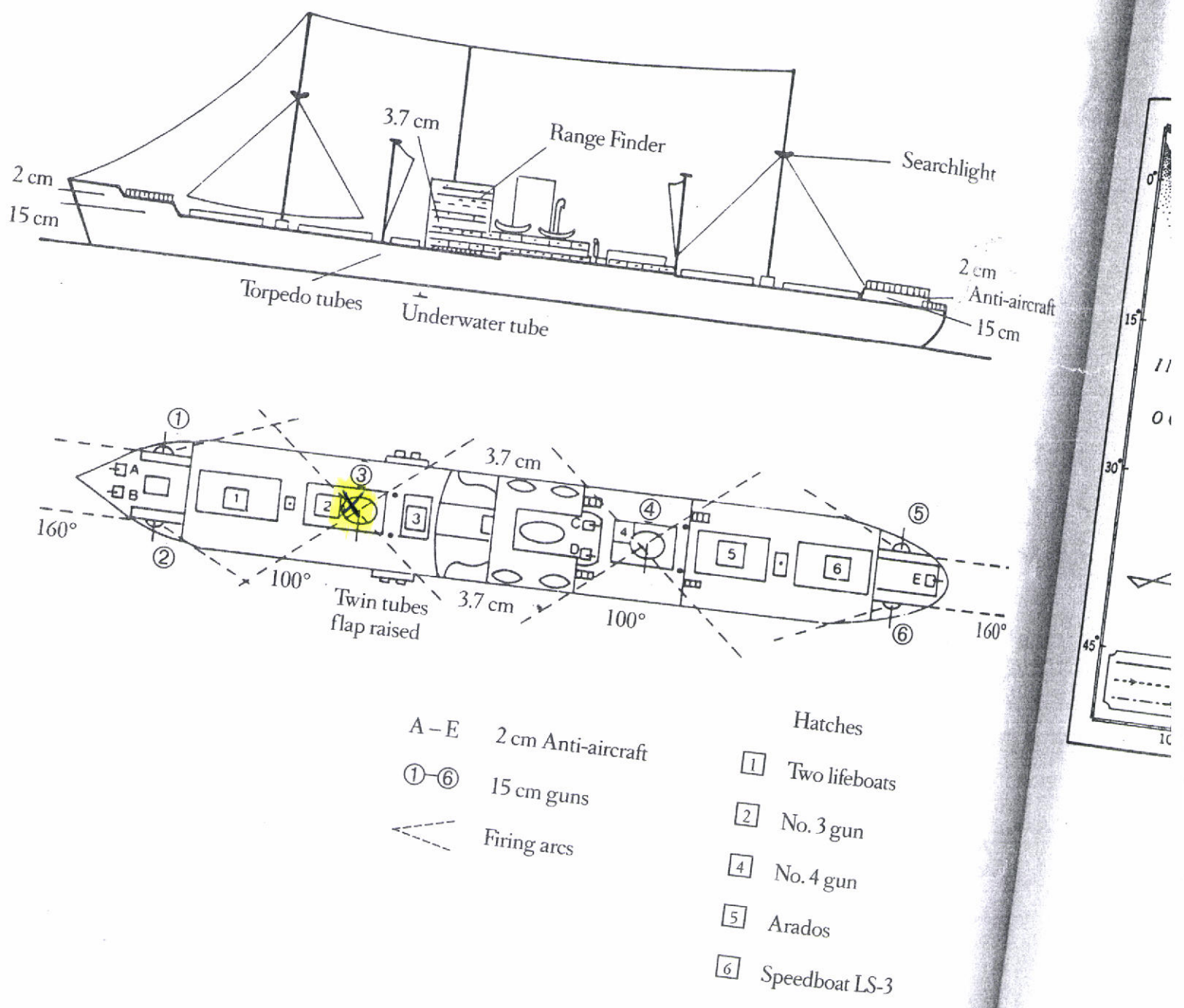
Figure 7 HSK Kormoran : side view and deck plan showing armaments
