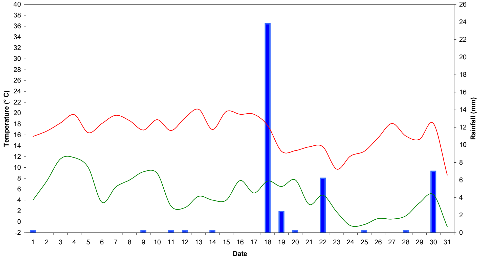
HQJOC AWS Temperature and rainfall - May 2007
