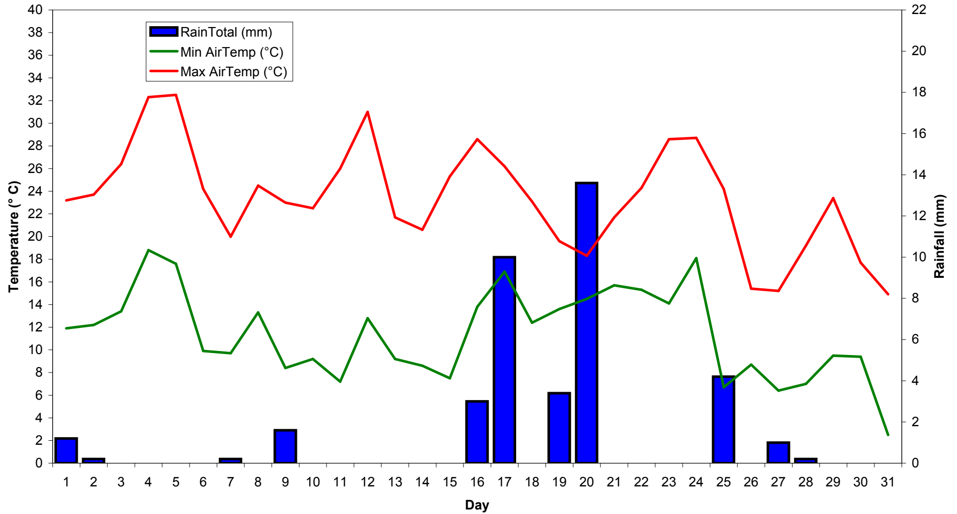
HQJOC AWS Temperature and Rainfall - March 2007
