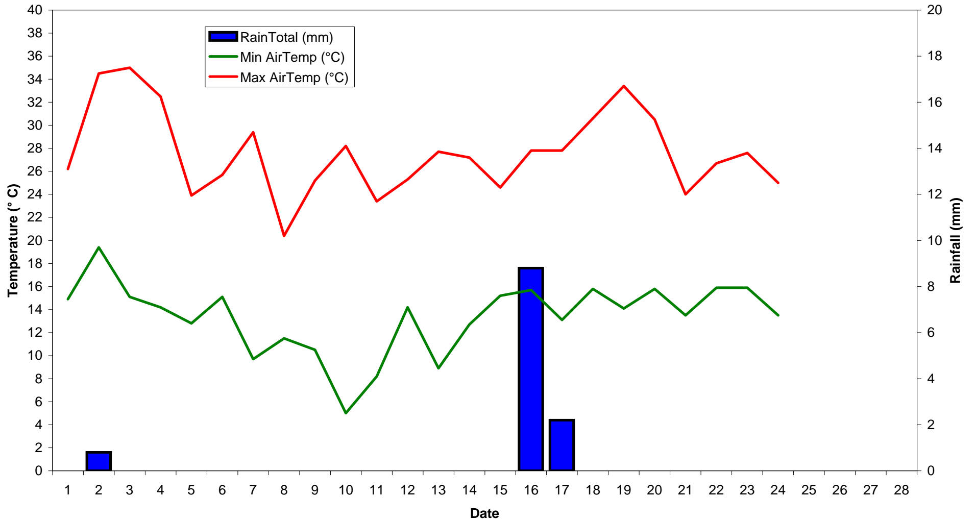
HQJOC AWS Temperature and rainfall - February 2006
