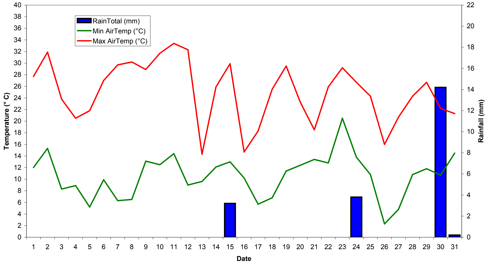
HQJOC AWS Temperature and rainfall - December 2006
