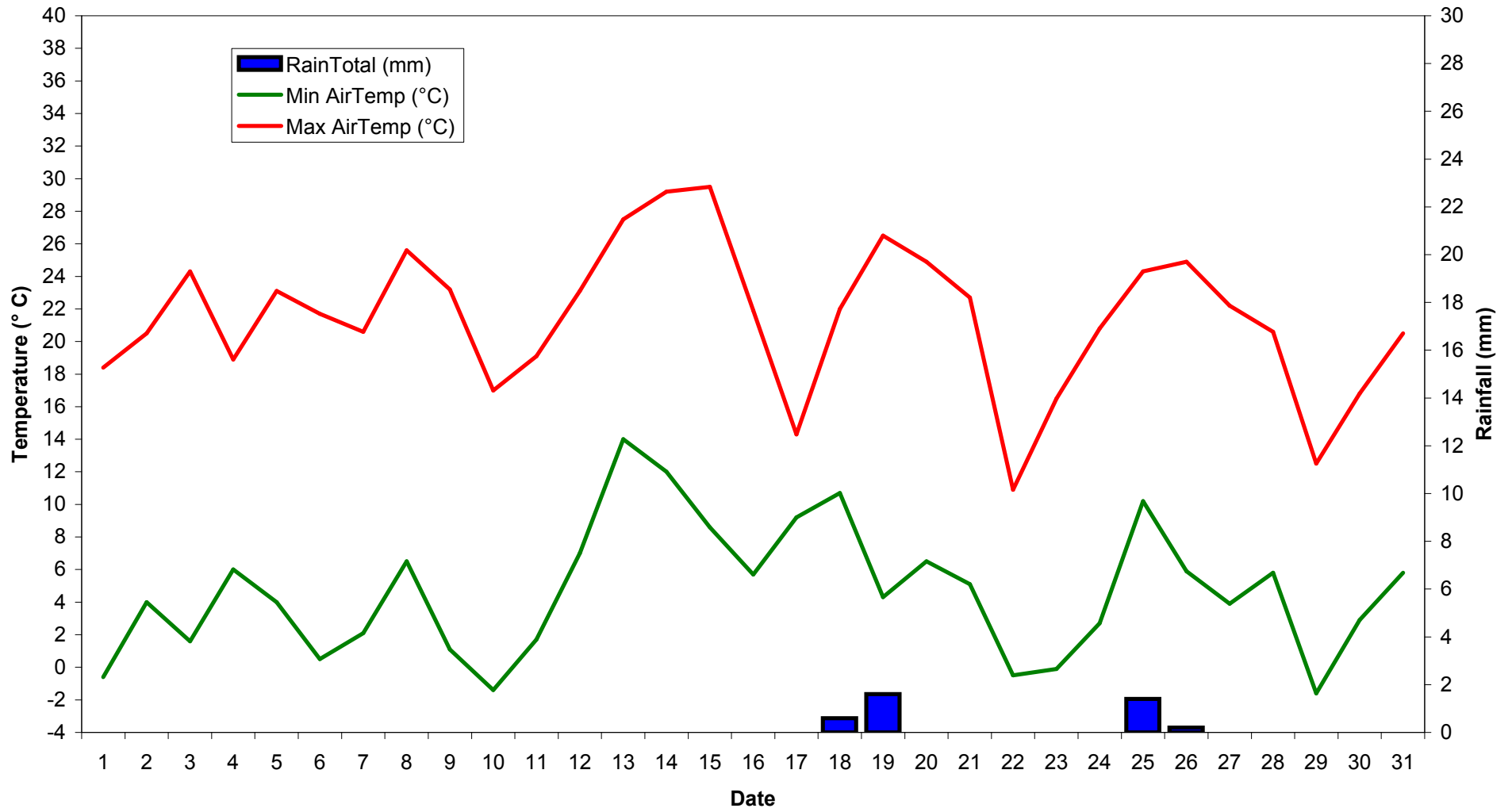
HQJOC AWS Temperature and rainfall - October 2006
